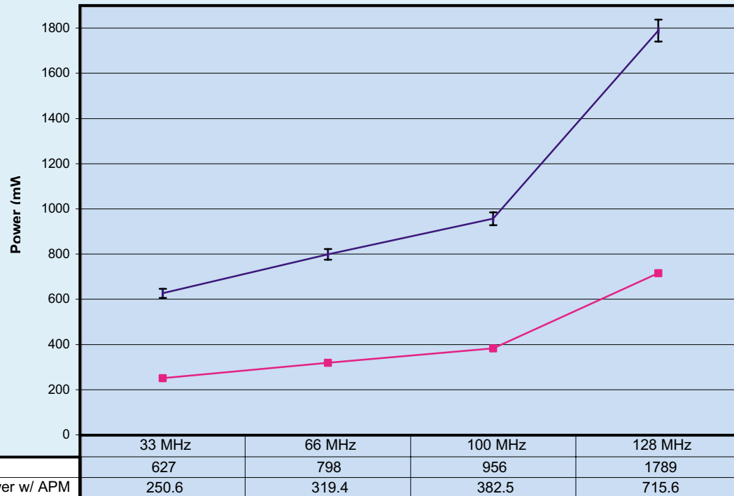
ZFx86 Core Power Consumption
